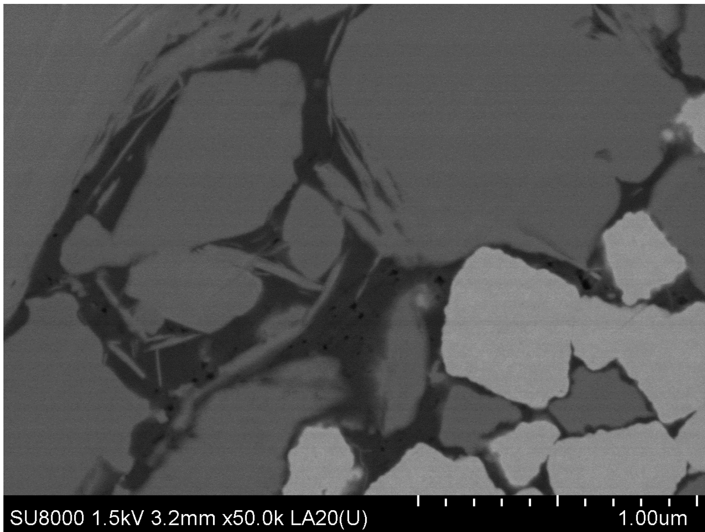
页岩气样品2: X50000
