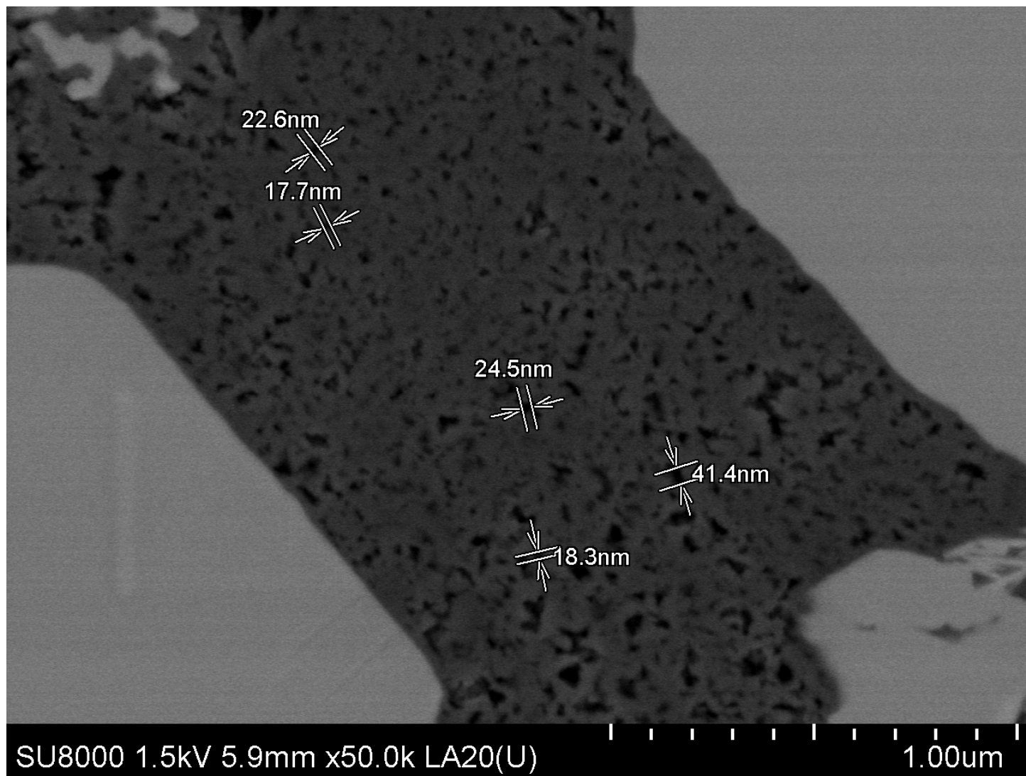
页岩气样品1: X50000
