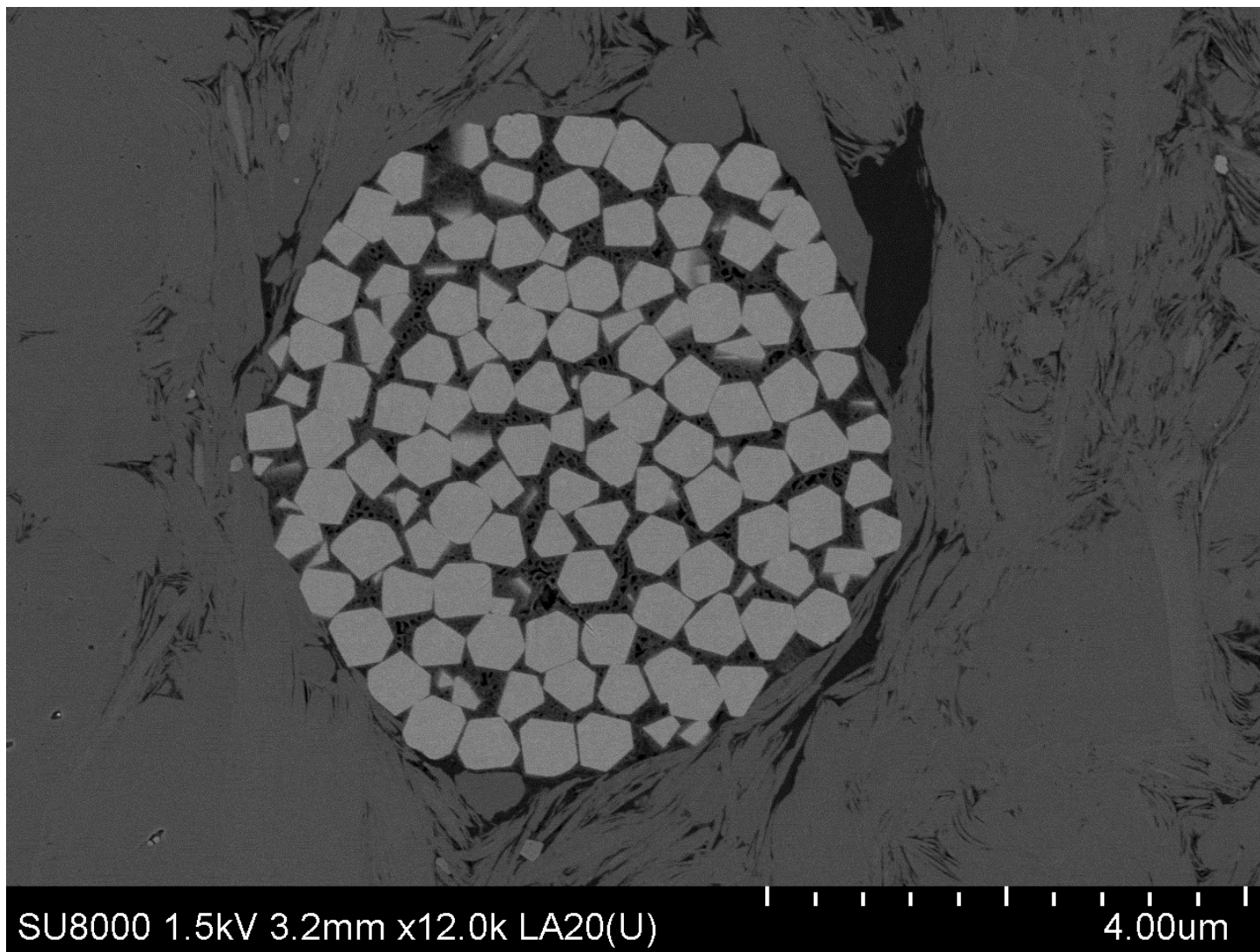
页岩气样品2: X12000
