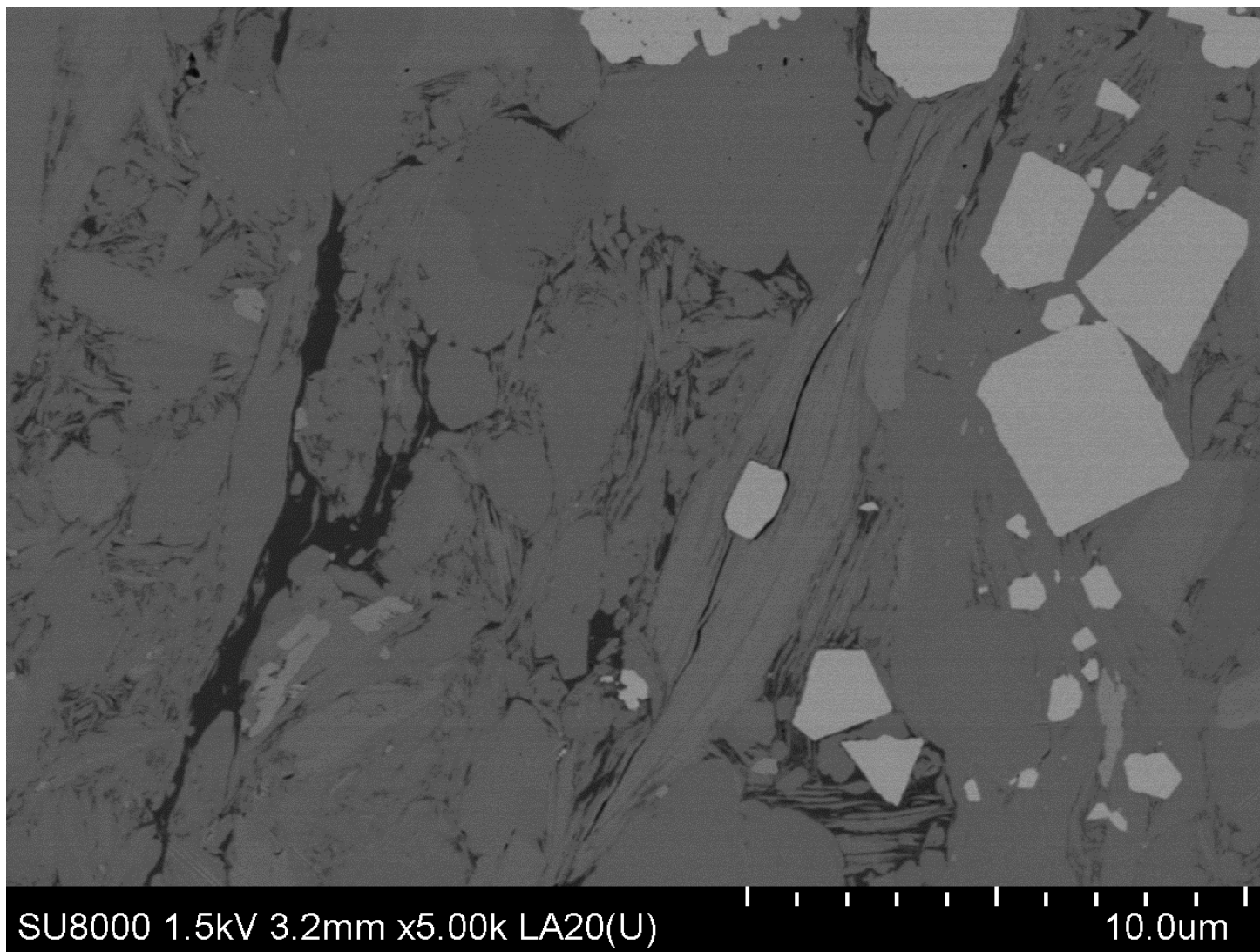
页岩气样品2: X5000
