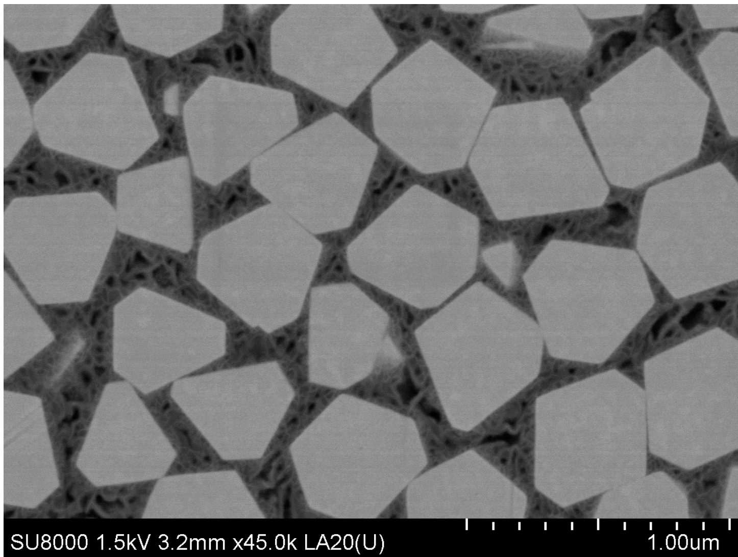
页岩气样品2: X45000
